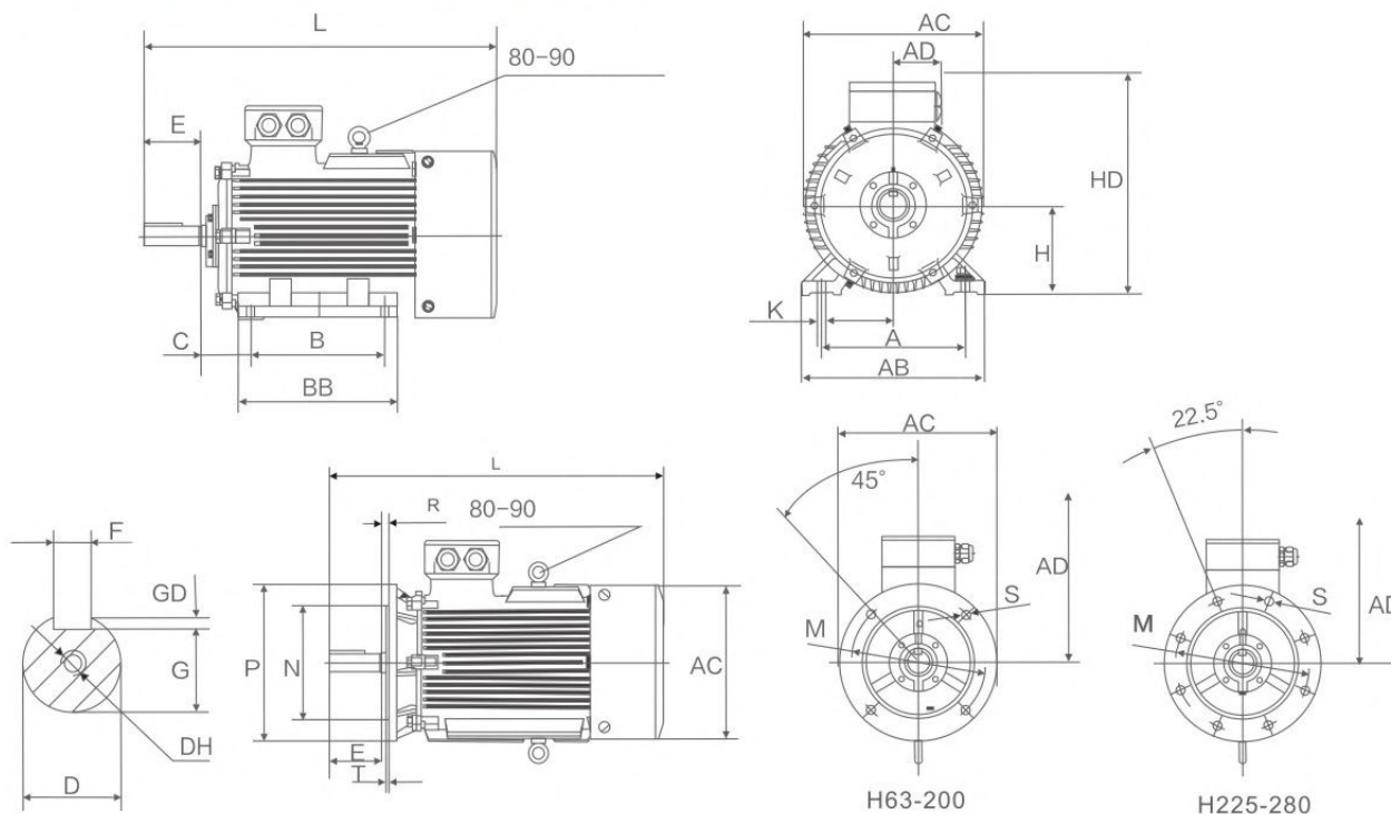
Mounting Dimensions
